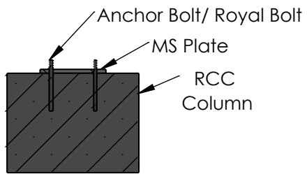
Cross section of column
