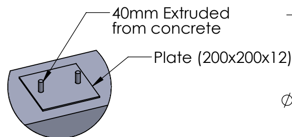
DETAIL C SCALE 1 : 12
